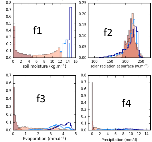
Simulation LmdzOrChoiAP for the region 60 Sahel (1980 - 1999)
